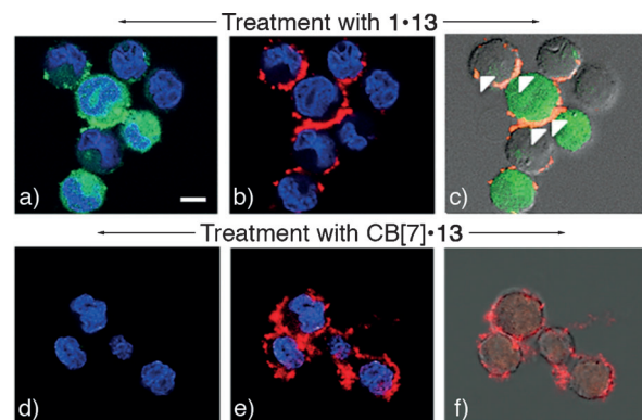
Figure 4. L1210FR cells that were incubated with 1 · 13 ( 15 \mu\text{M} , a–c) or CB[7]· 13 ( 15 \mu\text{M} , panels d–f) indicated receptor-specific uptake. L1210FR cells were treated with Dextran-Alexa Fluor 647 ( 125 \mu\text{g mL}^{-1} ) overnight followed by 1 · 13 or CB[7]· 13 the next day. Color code: 1 · 13 or CB[7]· 13 , green; Hoechst 33342 (nuclear stain), blue; dextran labeled with Alexa Fluor 647 (lysosome/endosome stain), red. a,d) Blue and green channels for cells treated with 1 · 13 or CB[7]· 13 . b,e) Blue and red channels for cells treated with 1 · 13 or CB[7]· 13 . c,f) Overlay of brightfield image, green and red channels for cells treated with 1 · 13 or CB[7]· 13 . The white arrows highlight yellow regions of colocalization of 1 · 13 and Dextran-Alexa Fluor 647. Scale bar = 5 \mu\text{m} applies to all images.
